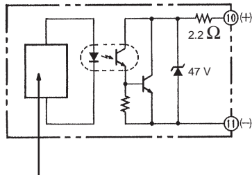
Main circuit of Sensor
