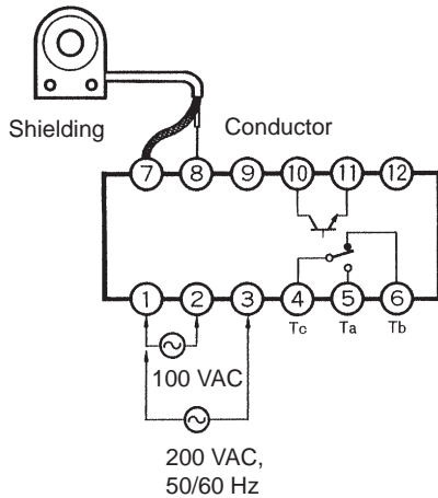
Main circuit of Sensor
