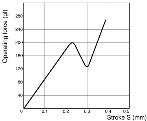
Operating Force vs. Stroke Characteristics B3WN-6002
